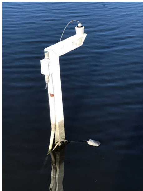
Photo: pump station with float switch
